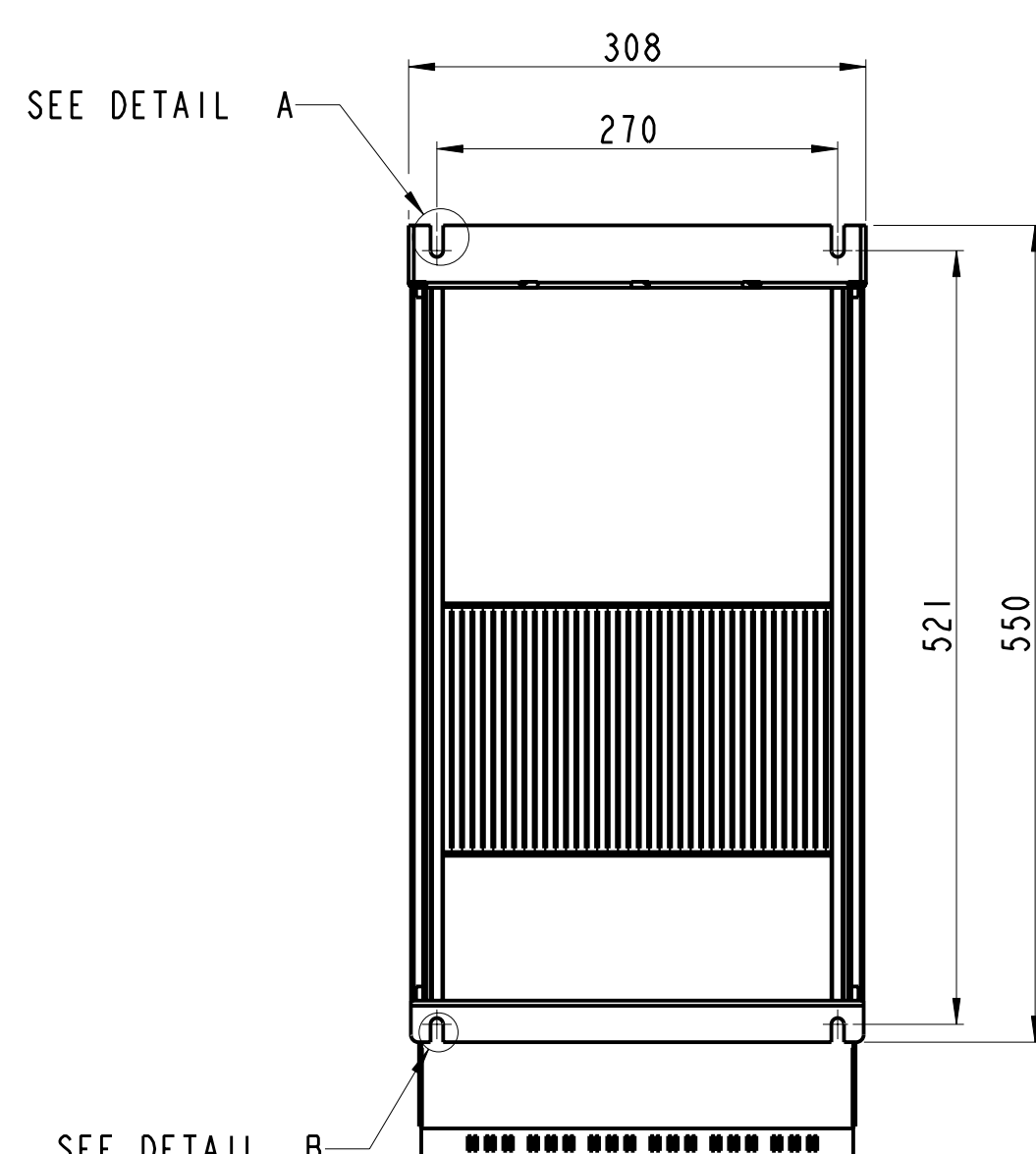
MOUNTING BASE
