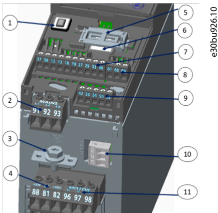
Illustration 35: Terminal Numbers
