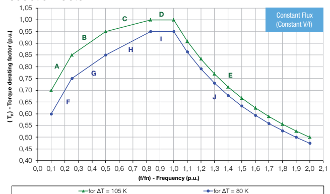
Figure 53 - Derating curve for motors driven by frequency inverter.
