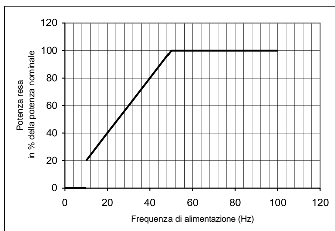
Fig. 2 - Power output - frequency diagram @ 50Hz
