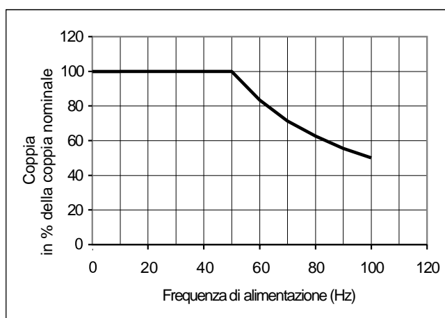
Fig. 3 - Torque - frequency diagram @ 50Hz
