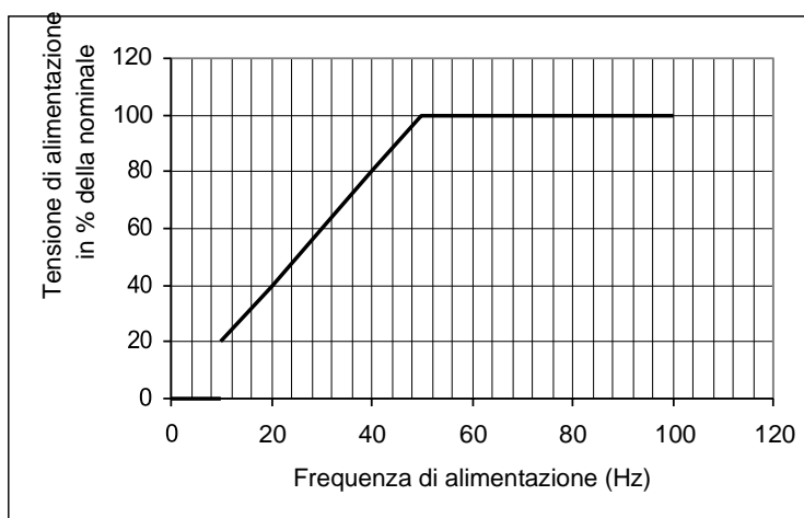
Diagr. 1 - Supply voltage - frequency diagram @ 50Hz
