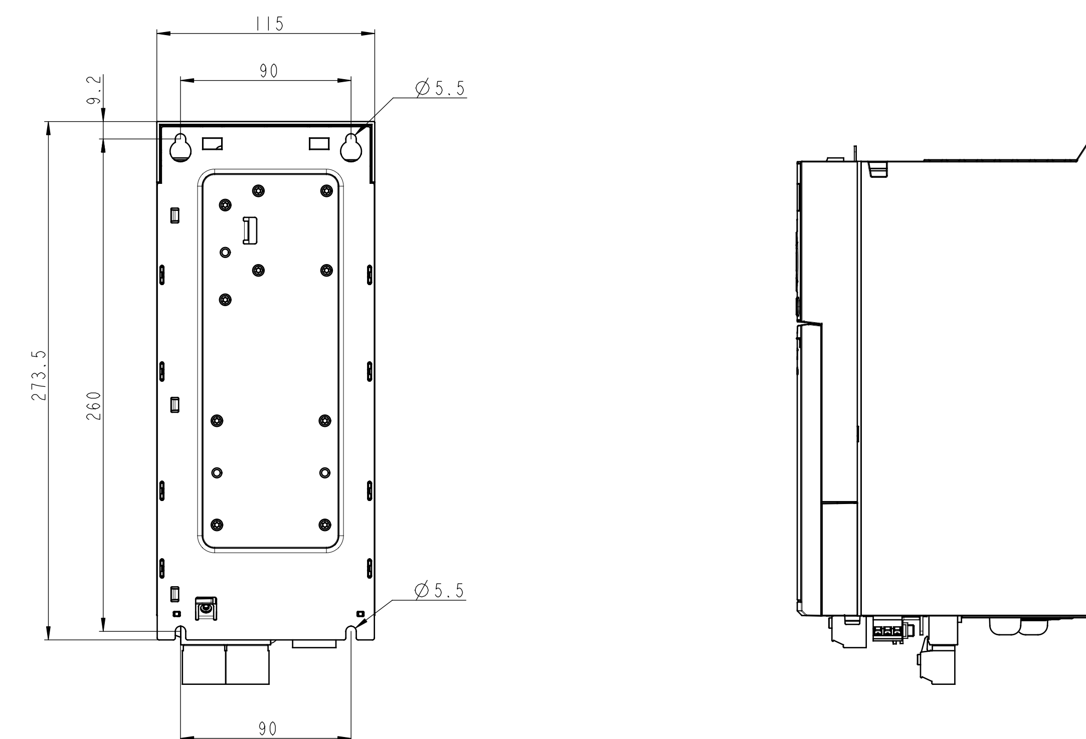
Mounting-Base
