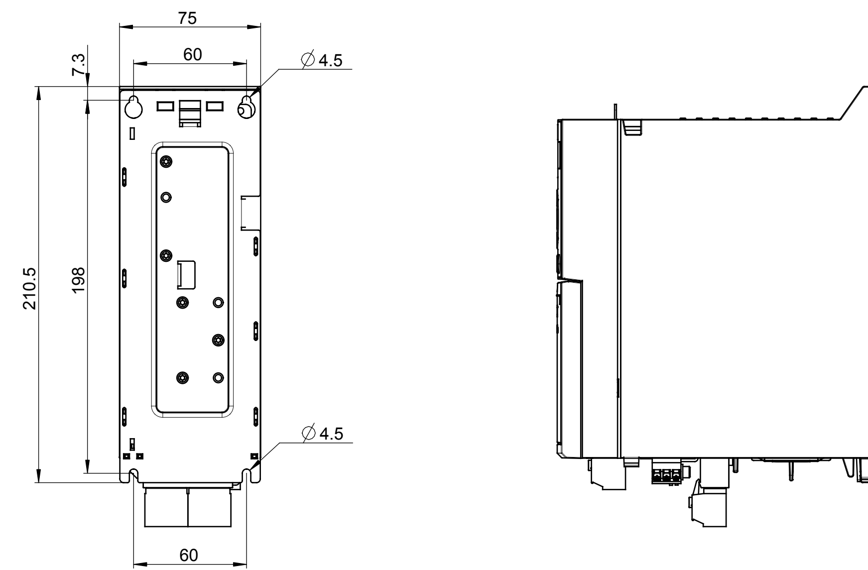
Mounting-Base
