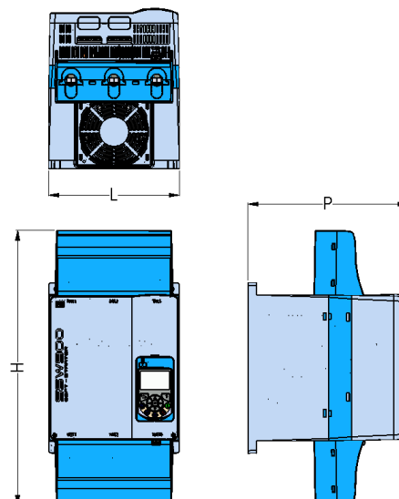
Figure 6.7: SSW0708900-IP20-4D
