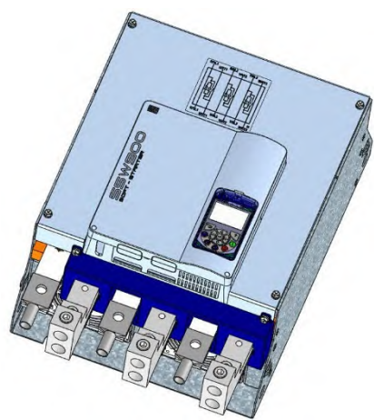
Figure 8.12: 1 x SSW900-3BAR-E-L
