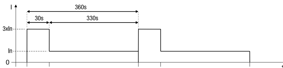
Figure 7.1: AC-53b:3-30:330
