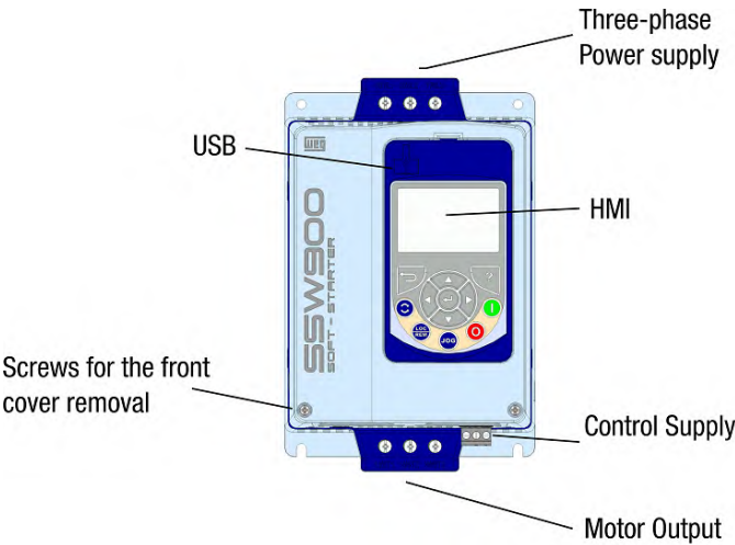
Figure 2.1: Front view of the SSW900
