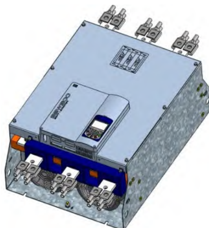
Figure 8.16: 2 x SSW900-3BAR-F-L
