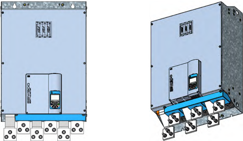
Figure 6.17: SSW900-3BAR-G
