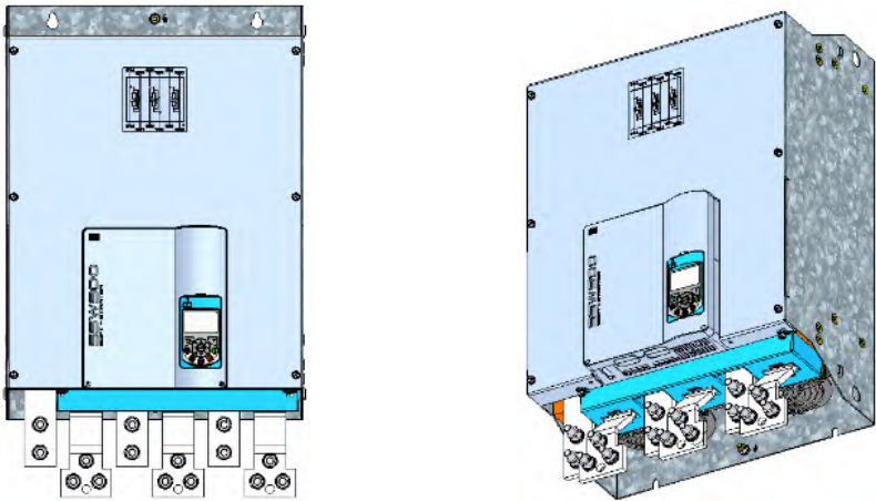
Figure 6.16: SSW900-3BAR-F-L45L
