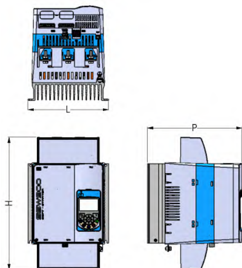
Figure 6.8: SSW0708900-PROT-3C
