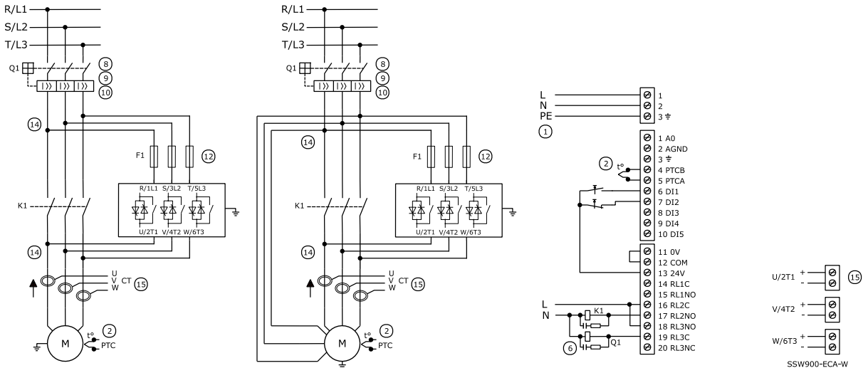
Standard Connection
