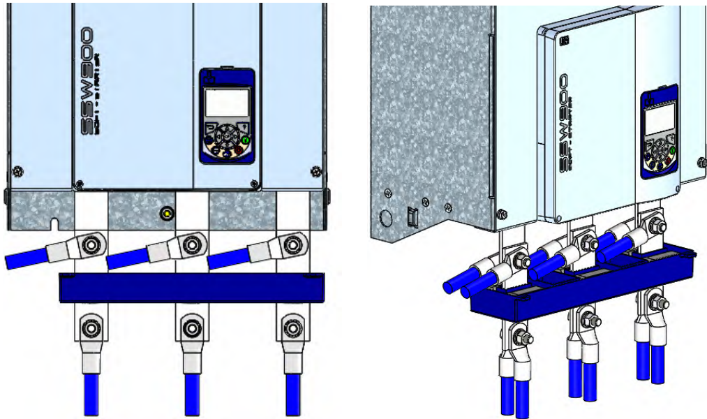
Figure 8.10: Cable Output Suggestion
