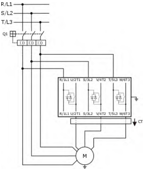
Standard feed
