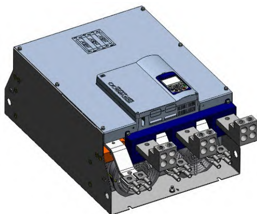
Figure 8.17: 1 x SSW900-3BAR-F-L45S
