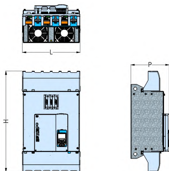
Figure 6.10: SSW900-PROT-E
