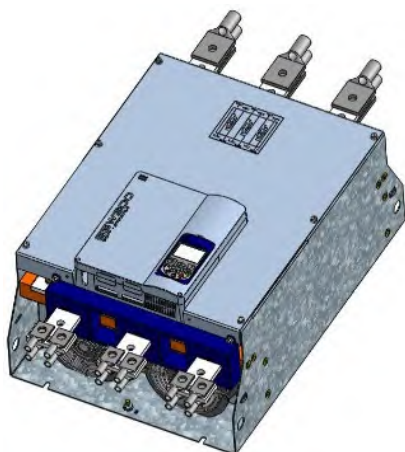
Figure 8.15: 1 x SSW900-3BAR-F-L
