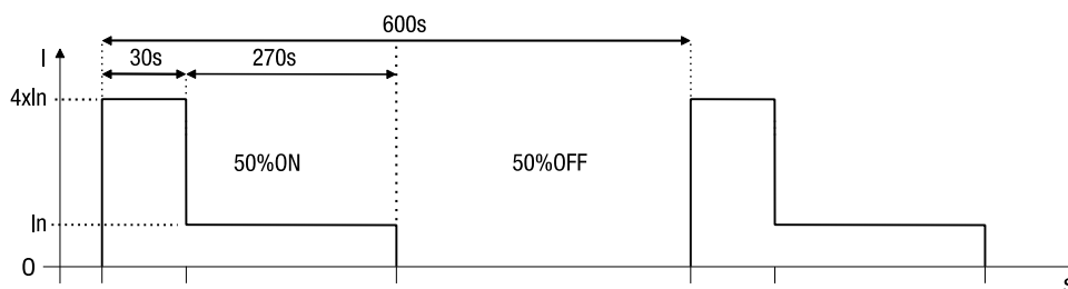
Figure 7.2: AC-53a:4-30:50-6
