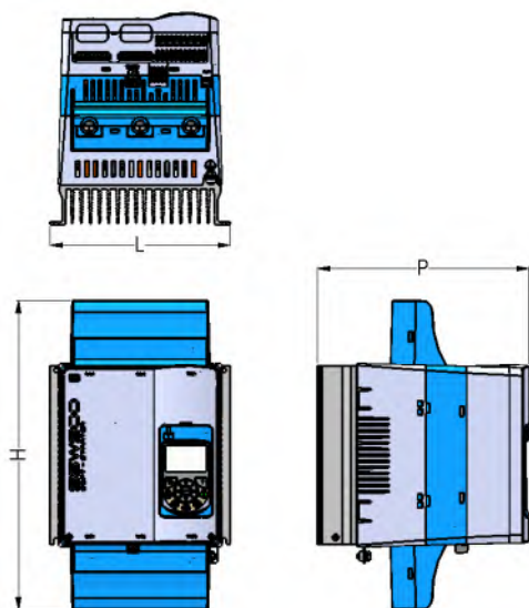
Figure 6.6: SSW0708900-IP20-3C
