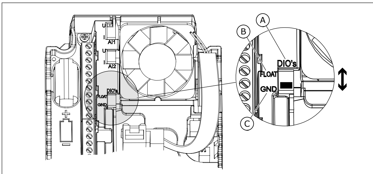
Afb. 7: DIP-switch
