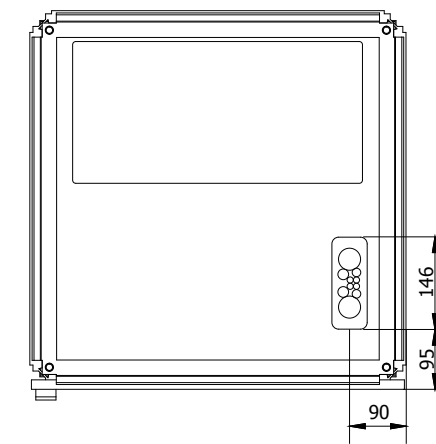
View B-B
