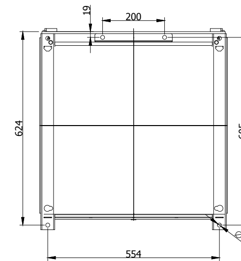
View C-C
