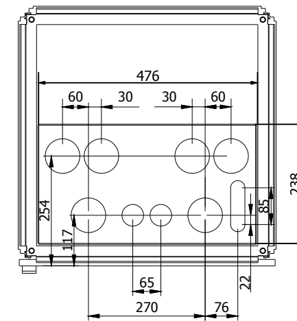
View C-C
