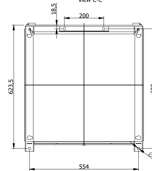
View C-C
