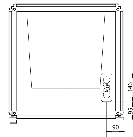
View B-B
