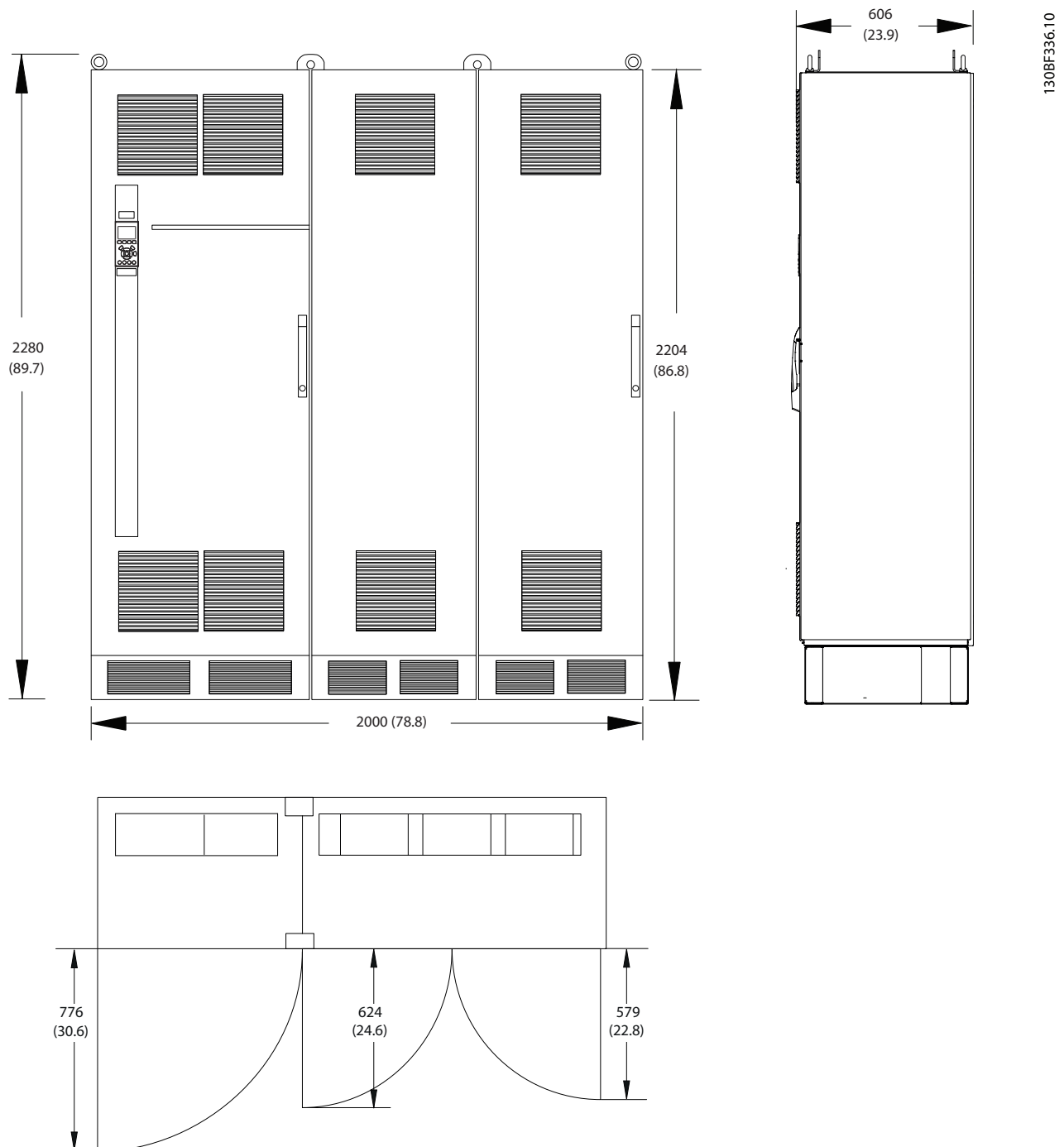
Figure 8.80 Front, Side, and Door Clearance Dimensions for F12
